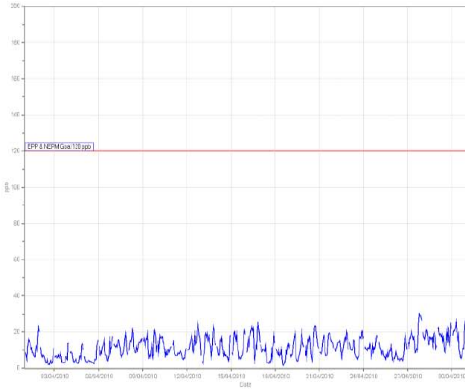
NO2[ppb] Station: LANDCENTRE Monthly: 04/2010 Type: AVG 1 Hr.
