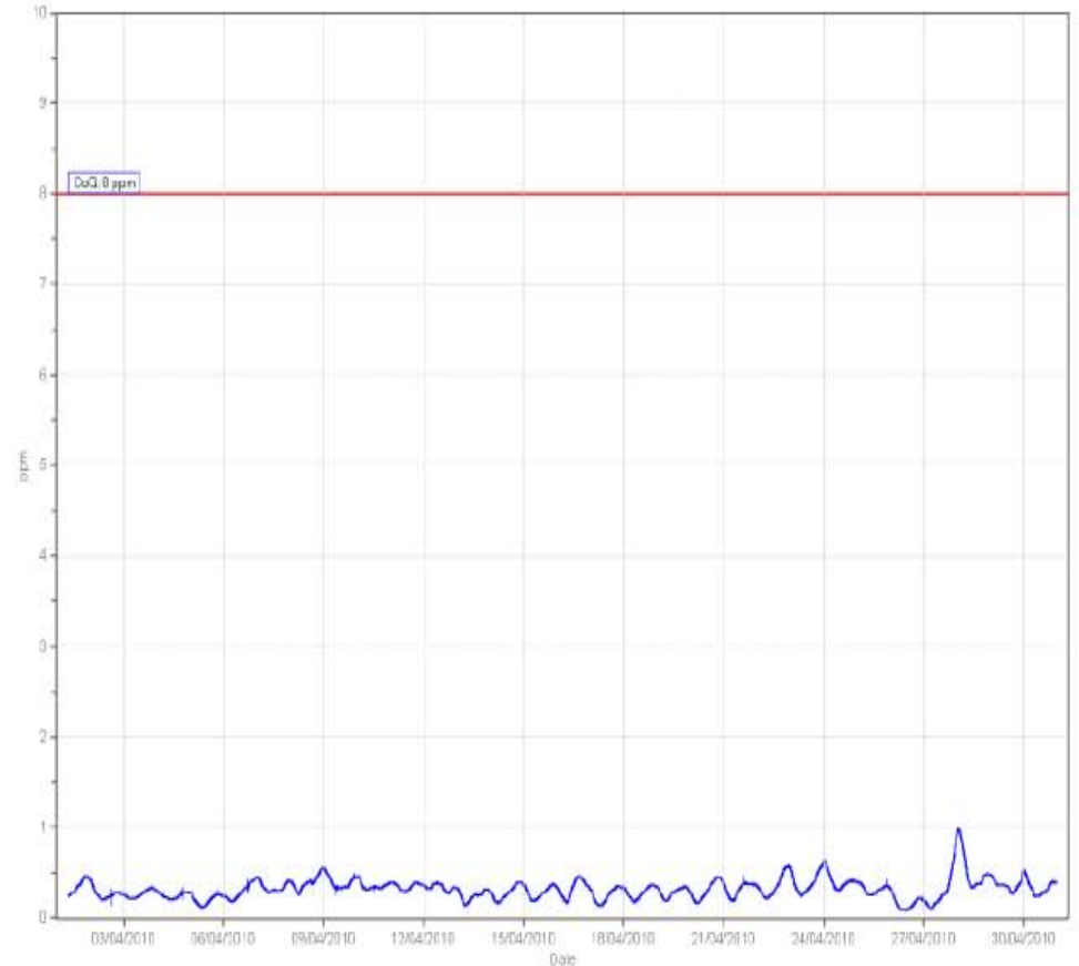
CO[ppm] Station: HAWTHORNE ST Monthly: 04/2010 Type: RunningAvg 8 Hrs.
