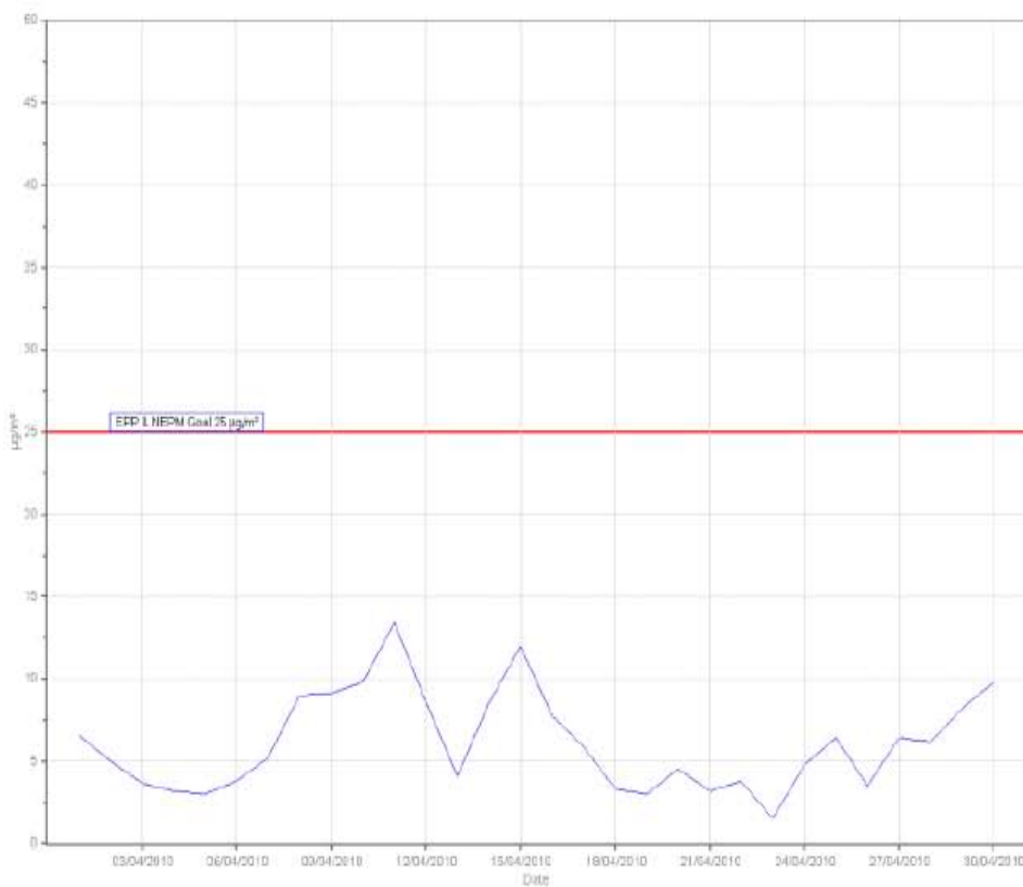
PM2.5_MC[µg/m 3 ] Station: LANDCENTRE Monthly: 04/2010 Type: AVG 1 Day
