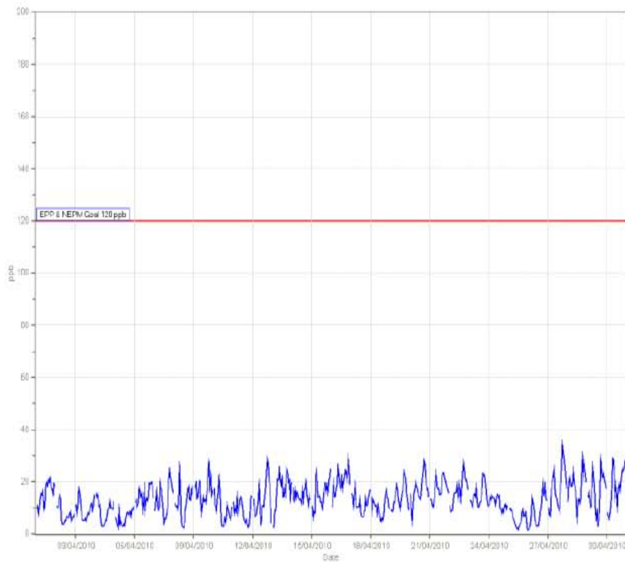
NO2[ppb] Station: NORTHEY Monthly: 04/2010 Type: AVG 1 Hr.
