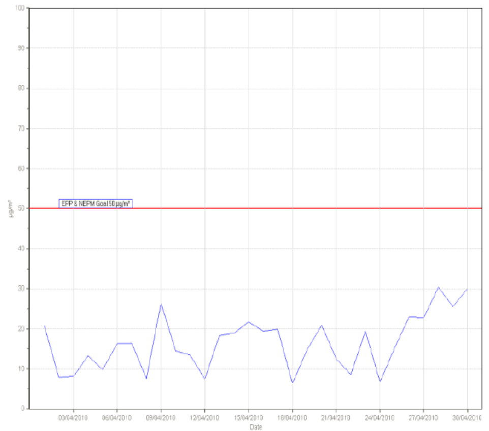
PM10[µg/m 3 ] Station: RBH Monthly: 04/2010 Type: AVG 1 Day
