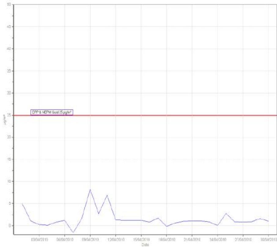
PM2.5_MC[µg/m 3 ] Station: NORTHEY Monthly: 04/2010 Type: AVG 1 Day
