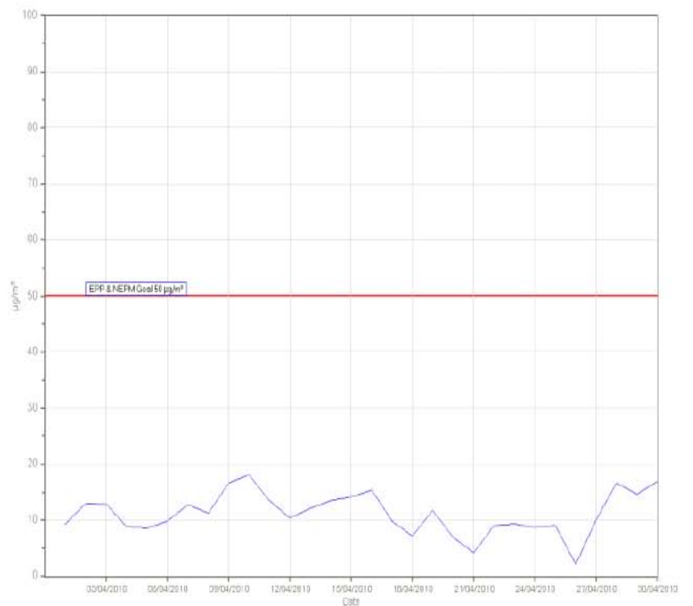
PM10[ug/m3] Station: HAWTHORNE ST Monthly: 04/2010 Type: AVG 1 Day
