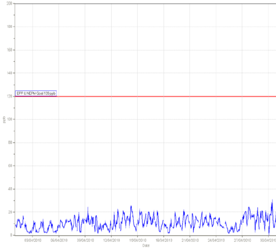
NO2[ppb] Station: RBH Monthly: 04/2010 Type: AVG 1 Hr.
