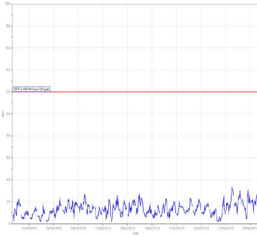
NO2[ppb] Station: HAWTHORNE ST Monthly: 04/2010 Type: AVG 1 Hr.
