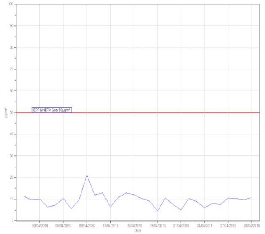
PM10[µg/m 3 ] Station: NORTHEY Monthly: 04/2010 Type: AVG 1 Day
