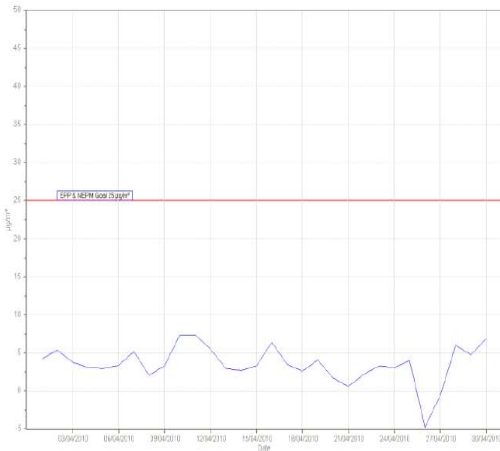
PM2.5_NC[ug/m3] Station: HAWTHORNE ST Monthly: 04/2010 Type: AVG 1 Day
