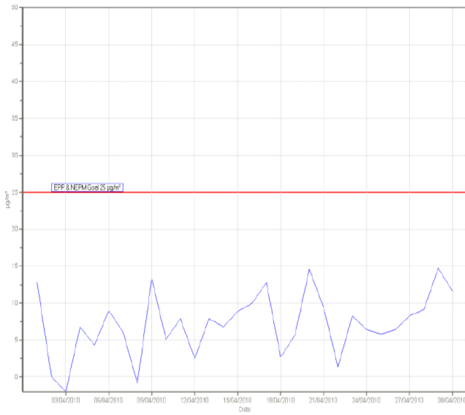
PM2.5_MC[µg/m 3 ] Station: RBH Monthly: 04/2010 Type: AVG 1 Day
